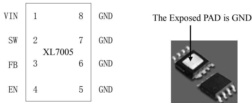
Figure2. Pin Configuration of XL7005 (Top View)
